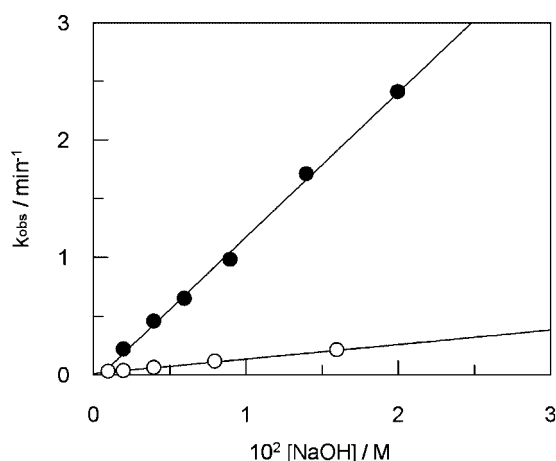
Figure 1. Influence of [NaOH] upon the pseudo first order rate constant of basic hydrolysis of CV (○) and MG (●) in water. T = 25^\circ\text{C}
