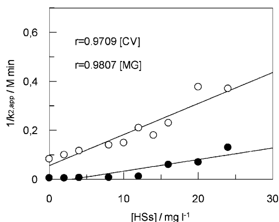
Figure 8. Fit of experimental data to Eqn (3). (○) CV and (●) MG. T = 25^{\circ}\text{C}
